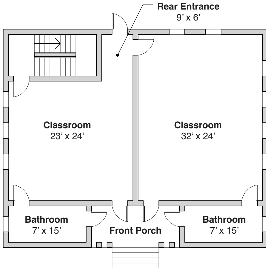
First Floor Plan 3/32" = 1'
